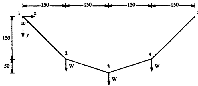
Fig. 4. Alternative experimental layout discussed in Section 4. All dimensions are in mm. The displacements which were measured after the r.h.s. cable had been shortened by 10 mm are given in Table 3.
